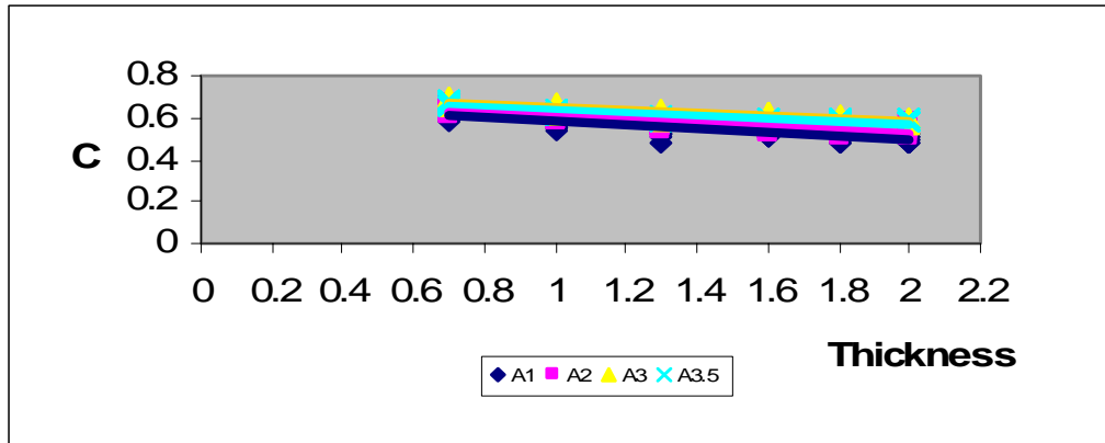
Fig.7 demonstrated contrast ratio (C) value for each ceramic shade as a function of thickness
