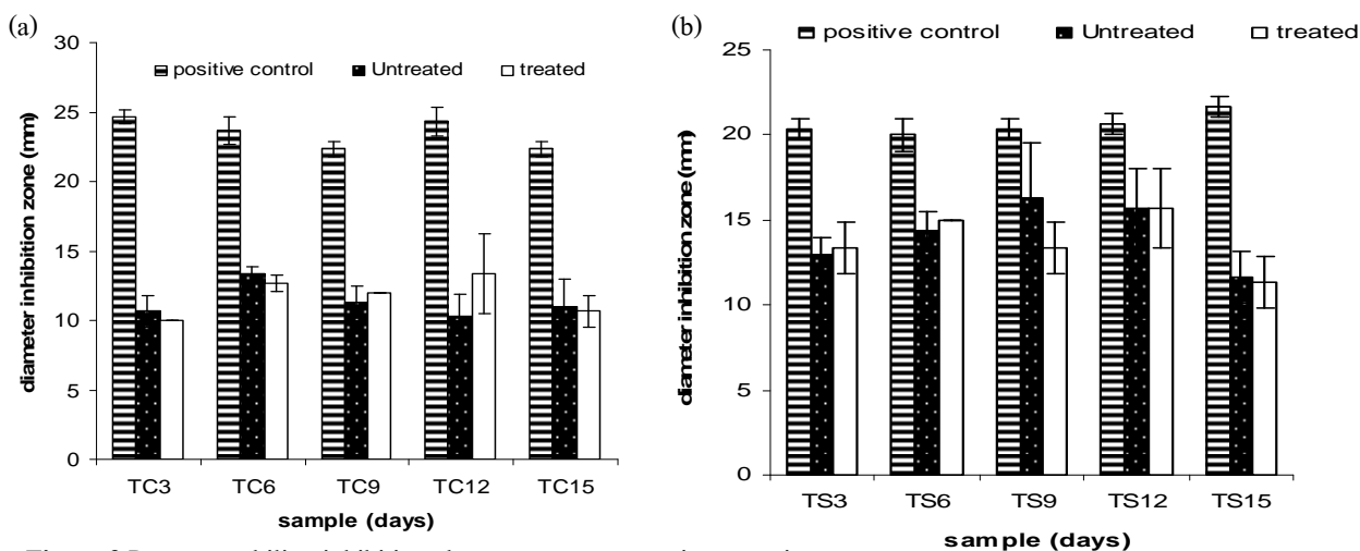
Figure 3 Pronase-stability, inhibition clear zone grown on microorganism
