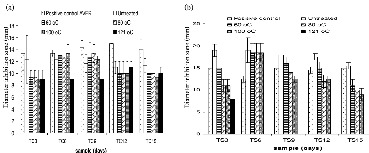
Figure 2 Thermal-stability, inhibition clear zone grown on microorganism
